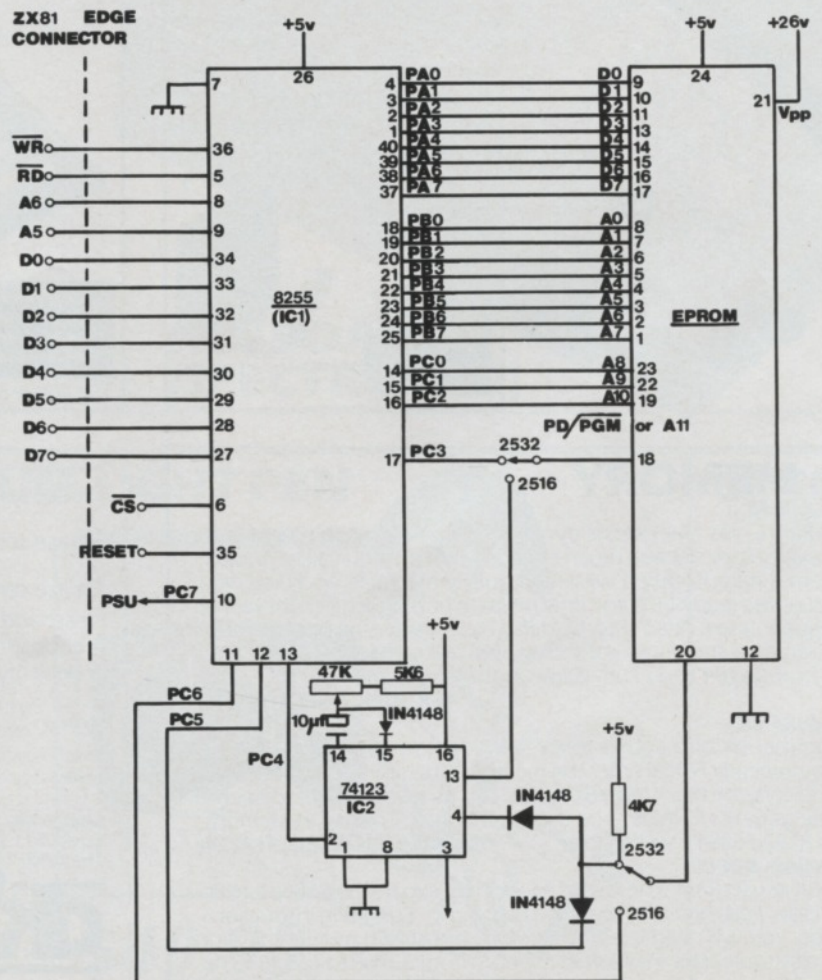
Figure 6: Main circuit diagram
